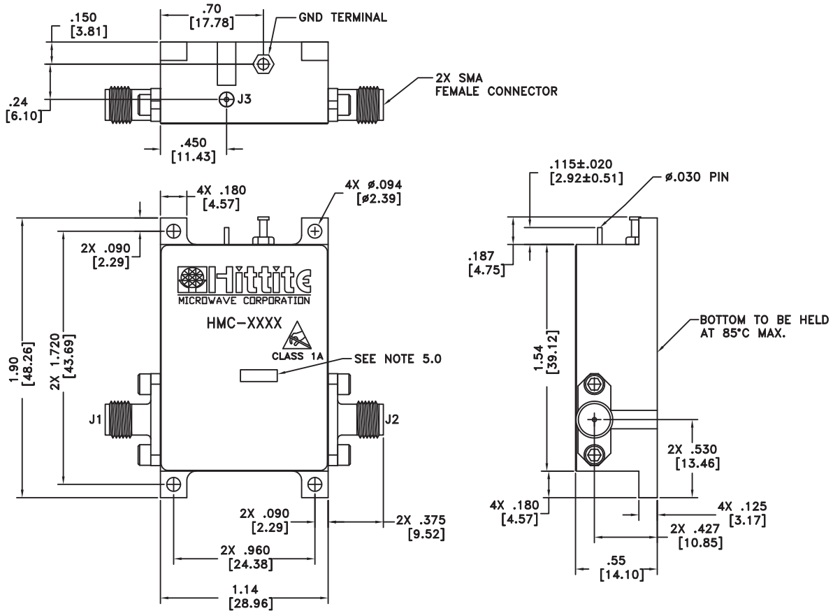
C-16 Package Outline Drawing
